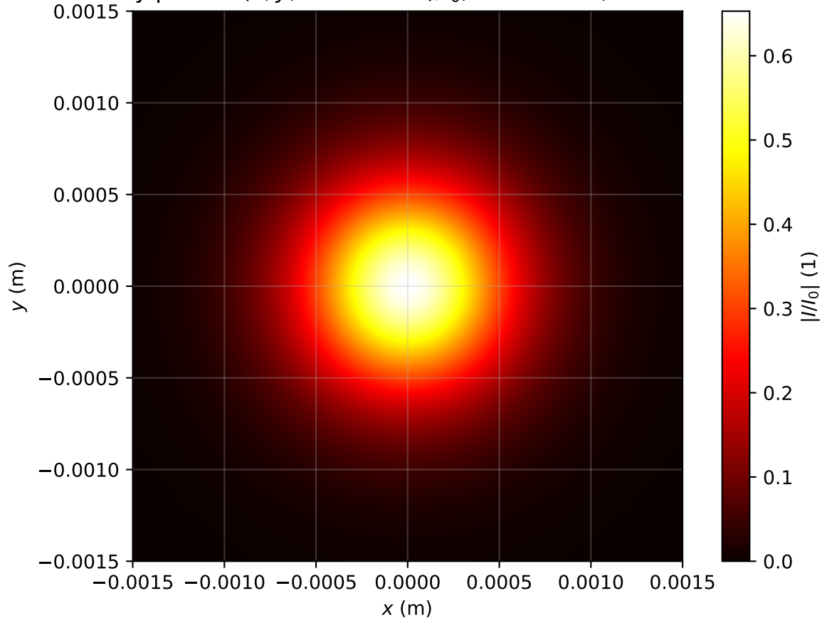
Intensity profile I(x, y, z = 3.105m)/I_0 , \text{Pin}=0.6\text{Pcr} , artificial time
